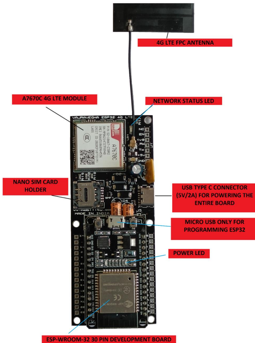
Module Board
